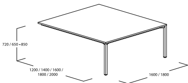
Bench Twin Baukasten - Endmodul
