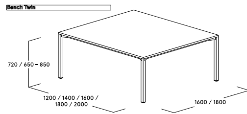
Bench Twin
